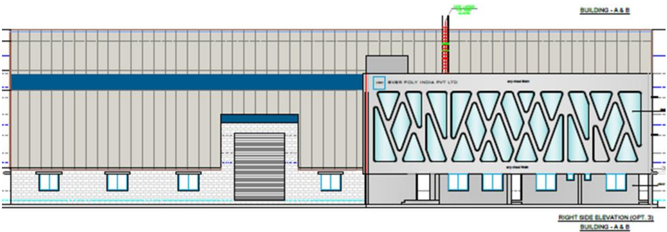
Factory for SVSR Polytex, Sanand (Gujarat)
